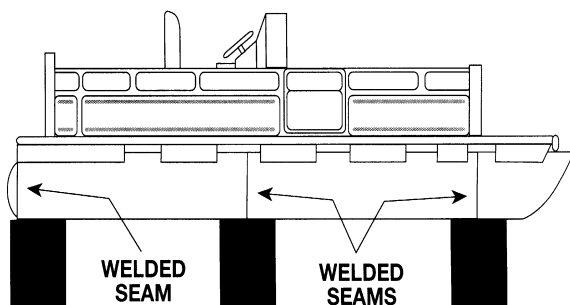
Figure 7-1 Pontoon Boat Storage Support
