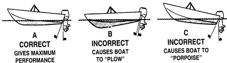
Figure 4-7 - Motor Angle
